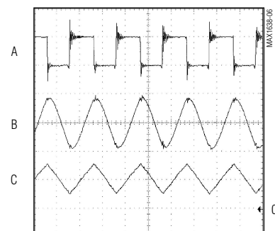
SWITCHING WAVEFORMS
