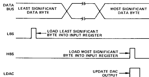
Figure 7. Timing Diagram
