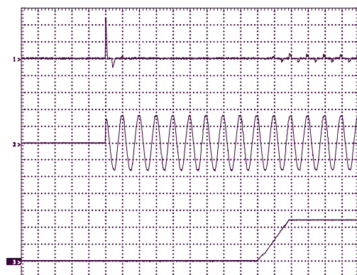
Fig. 6-1 Input inrush current, typical behavior
