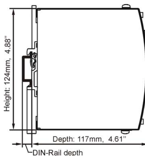
Fig. 23-2 Side view
