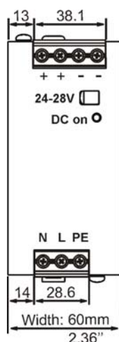
Fig. 23-1 Front view
