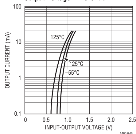
LT1460S3-10V Minimum Input-Output Voltage Differential
