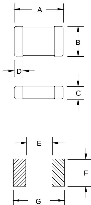
Pad Layout
