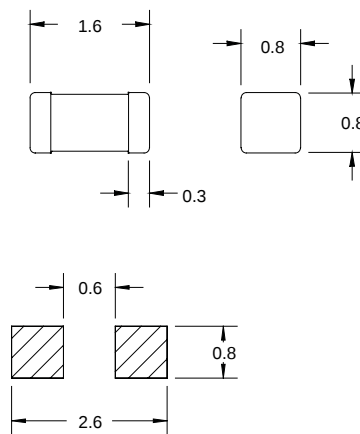
Pad Layout
