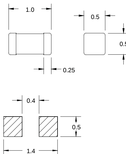
Pad Layout
