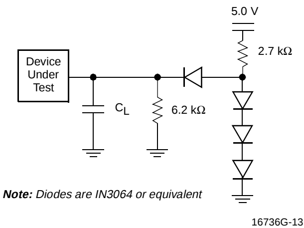
Figure 7. Test Setup
