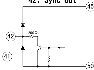
42; Sync out
