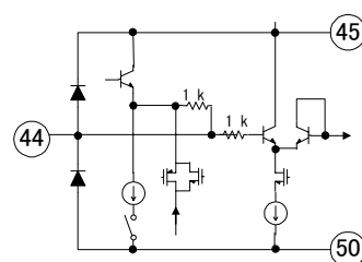
44; Y3/CVBS3 in
