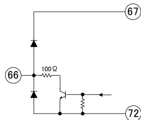
66: DAC 3
