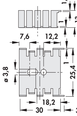
FK 216 CB ... 15 K/W
