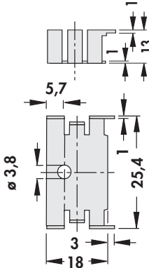
FK 215 32 ... 21 K/W
