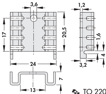
FK 232 220 ...
