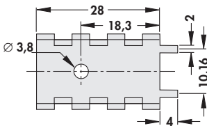
FK 235 L 1 ... TO 220
