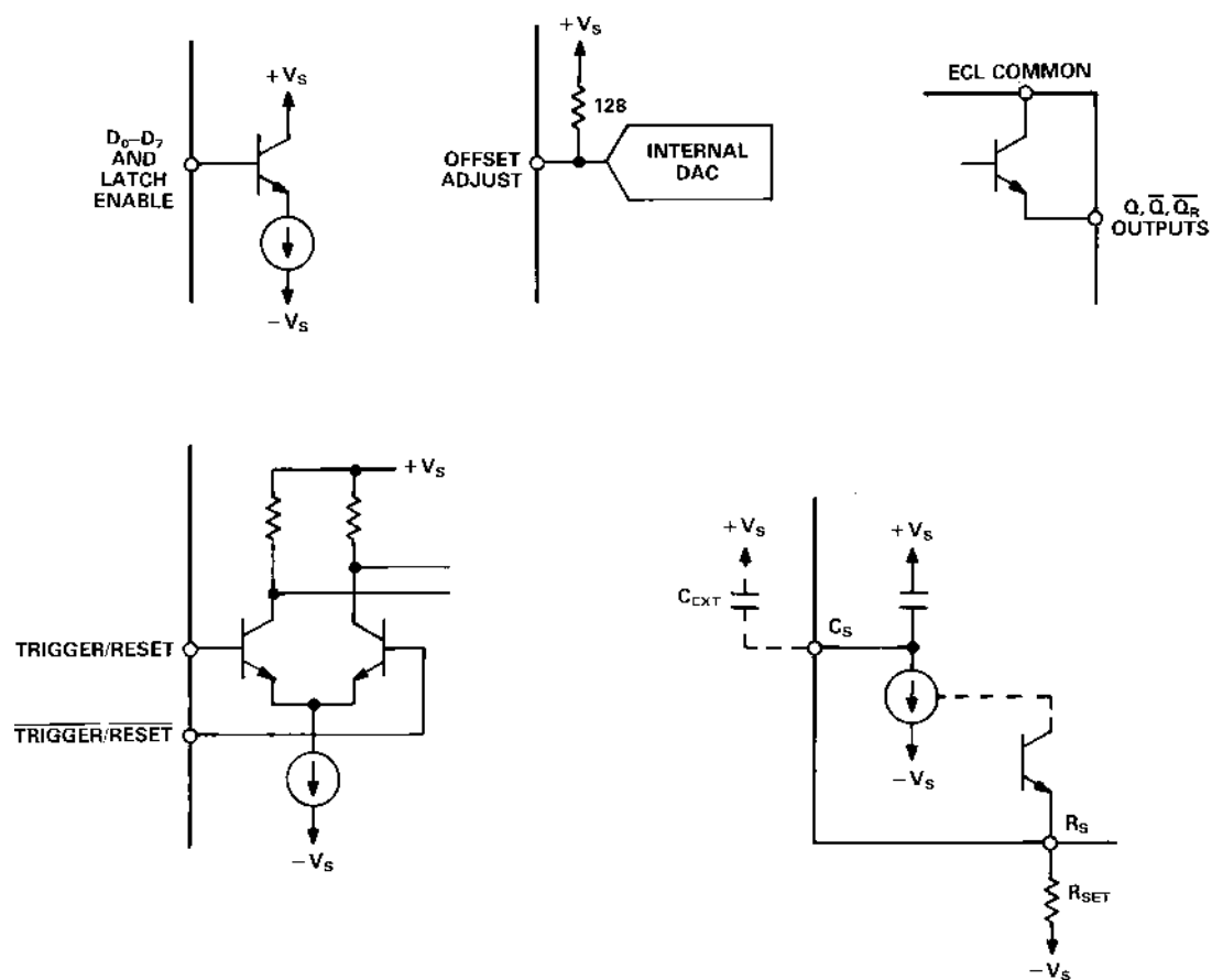
Figure 2. Input/Output Circuits
