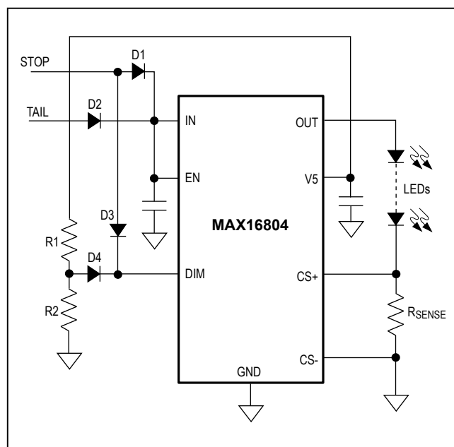
Figure 2. Two-Level Brightness Operation
