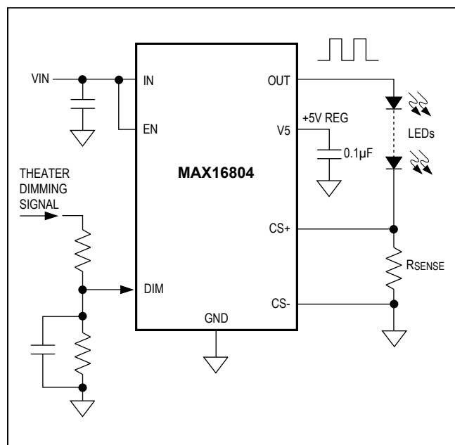
Figure 1. Theater Dimming
