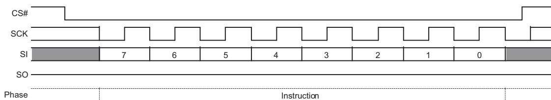
Figure 9.3 Write Enable (WREN 06h) Command Sequence
