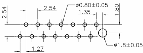
PCB Layout
