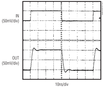
MAX4314 SMALL-SIGNAL PULSE RESPONSE
