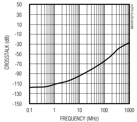
MAX4310/MAX4313 All-HOSTILE CROSSTALK vs. FREQUENCY
