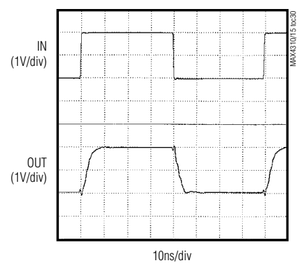
MAX4310 LARGE-SIGNAL PULSE RESPONSE
