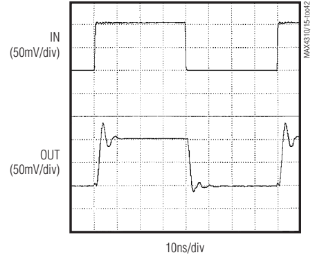
MAX4310 SMALL-SIGNAL PULSE RESPONSE ( C_L = 10pF )
