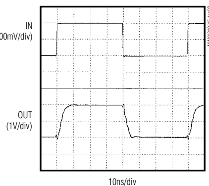
MAX4313 LARGE-SIGNAL PULSE RESPONSE
