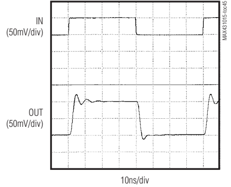
MAX4313 SMALL-SIGNAL PULSE RESPONSE ( C_L = 22pF )
