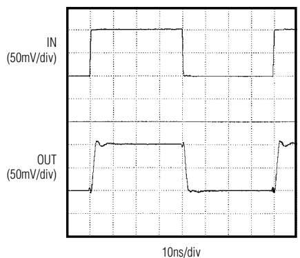
MAX4310 SMALL-SIGNAL PULSE RESPONSE
