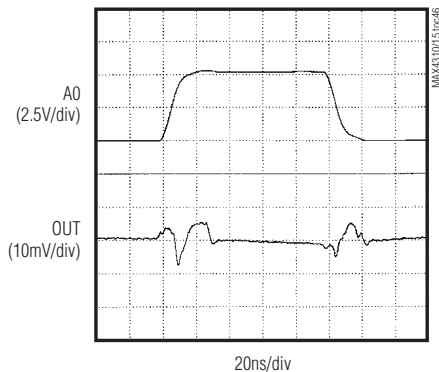
CHANNEL-SWITCHING TRANSIENT
