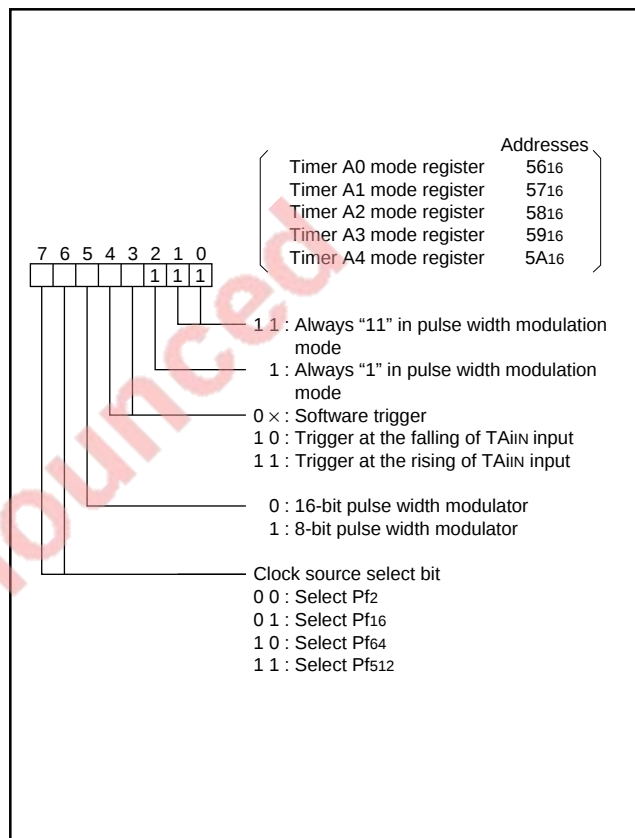
Fig. 32 Timer Ai mode register bit configuration during pulse width modulation mode
