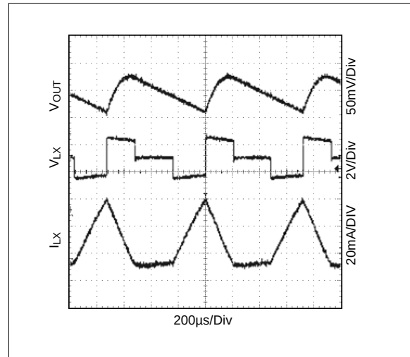
Figure 16. Switching Waveform; V_{OUT} = 2.7V
