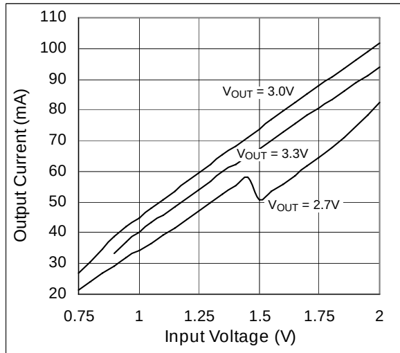
Figure 15. Output Current vs. Input Voltage
