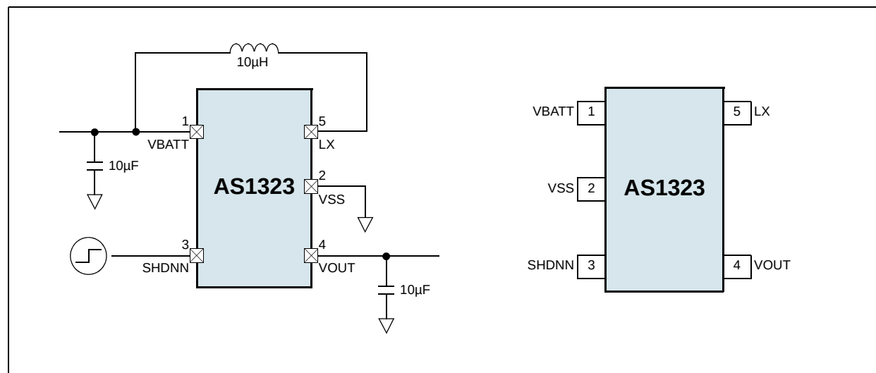
Figure 1. Typical Operating Circuit
