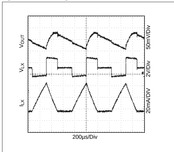
Figure 17. Switching Waveform; V_{OUT} = 3.0V
