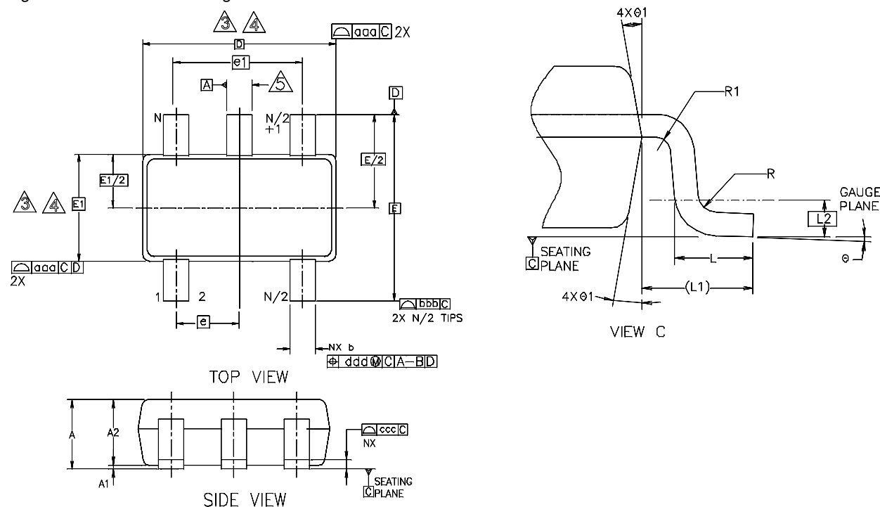
Figure 21. TSOT23-5 Package
