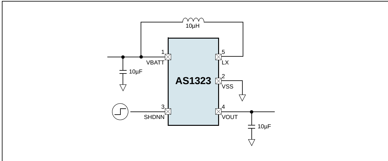
Figure 20. Typical Application
