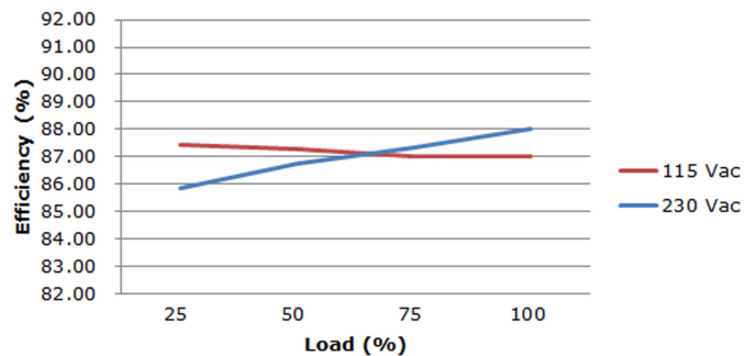
VOF-50B-15 Efficiency vs. Output Load (Natural Convection)
