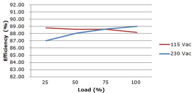
VOF-50B-24 Efficiency vs. Output Load (Natural Convection)
