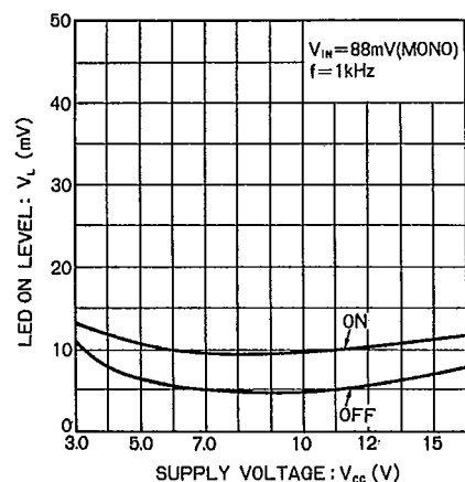
Fig. 15 LED 点灯入力電圧—電源電圧
