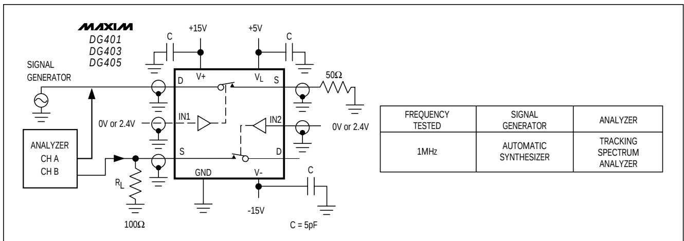
Figure 6. Crosstalk
