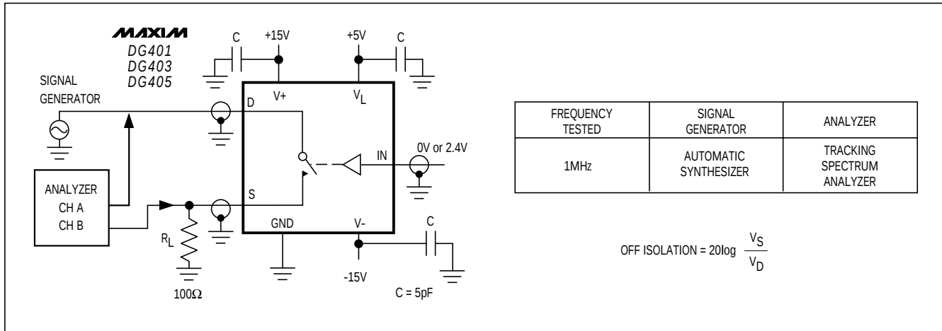
Figure 5. Off Isolation
