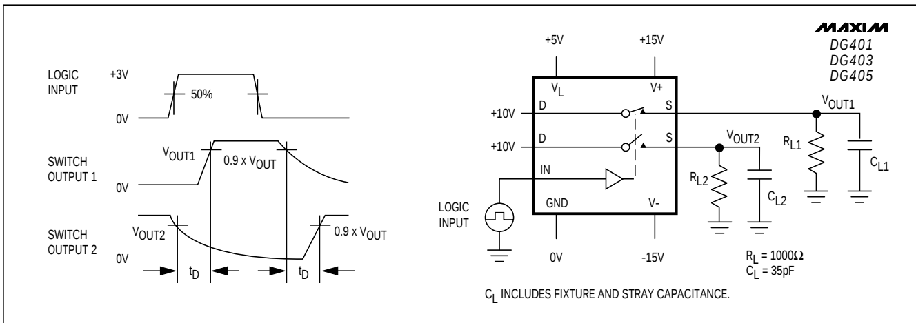
Figure 3. Break-Before-Make Interval
