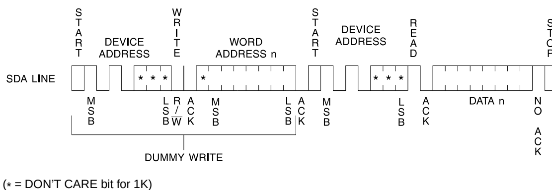
Figure 5. Random Read
