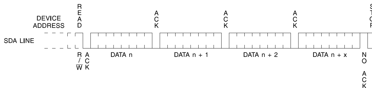
Figure 6. Sequential Read
