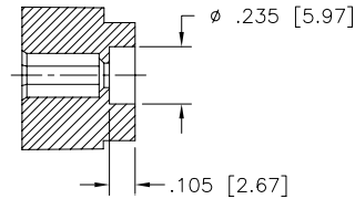
SECTION U-U
