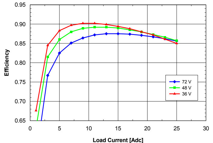
Fig. 2.5V.2: Efficiency vs. load current and input voltage for SQM48T/S25025 converter mounted vertically with air flowing from pin 3 to pin 1 at a rate of 300 LFM (1.5 m/s) and T_a = 25^{\circ}\text{C} .
