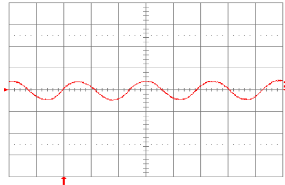
Fig. 2.5V.9: Input reflected ripple current, i_c (100 mA/div.), measured at input terminals at full rated load current and V_{in} = 48\ \text{V} . Refer to Fig. 2.5V.8 for test setup. Time scale: 1\ \mu\text{s}/\text{div} .
