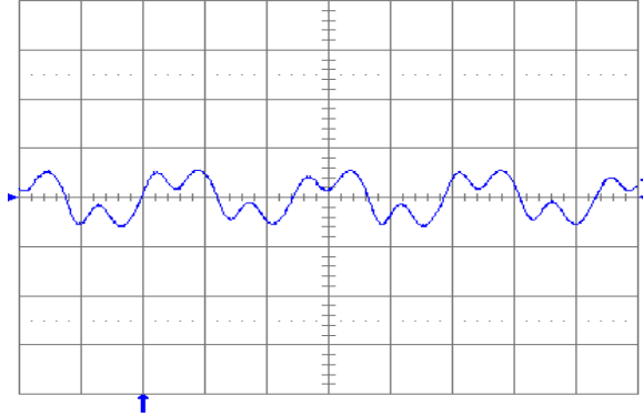
Fig. 2.5V.7: Output voltage ripple (20 mV/div.) at full rated load current into a resistive load with C_o = 10\ \mu\text{F} tantalum + 1\ \mu\text{F} ceramic and V_{in} = 48\ \text{V} . Time scale: 1\ \mu\text{s}/\text{div} .
