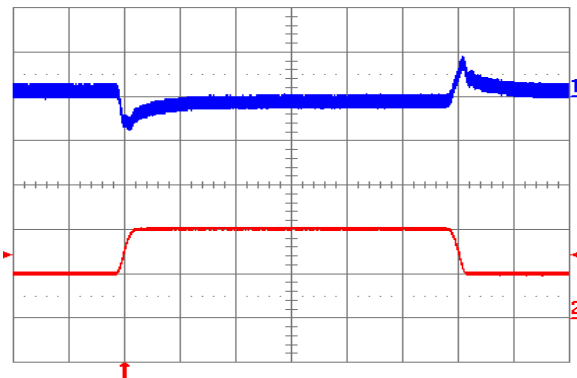
Fig. 1.8V.5: Output voltage response to load current step-change (5 A – 10 A – 5 A) at V_{in} = 48 V. Top trace: output voltage (100 mV/div.). Bottom trace: load current (5 A/div.). Current slew rate: 0.1 A/ \mu s. C_o = 1 \mu F ceramic. Time scale: 0.2 ms/div.
