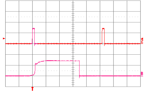
Fig. 1.2V.12: Load current (top trace, 20 A/div., 20 ms/div.) into a 10 mΩ short circuit during restart, at Vin = 48 V. Bottom trace (20 A/div., 1 ms/div.) is an expansion of the on-time portion of the top trace..
