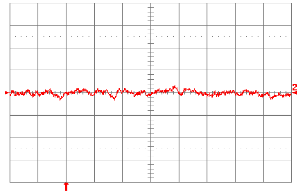
Fig. 2.5V.10: Input reflected ripple current, i_s (10 mA/div.), measured through 10\ \mu\text{H} at the source at full rated load current and V_{in} = 48\ \text{V} . Refer to Fig. 2.5V.8 for test setup. Time scale: 1\ \mu\text{s}/\text{div} .
