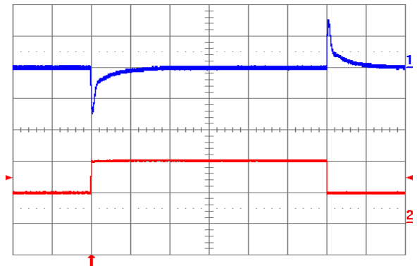
Fig. 1.2V.6: Output voltage response to load current step-change (5 A – 10 A – 5 A) at V_{in} = 48 V. Top trace: output voltage (100 mV/div.). Bottom trace: load current (5 A/div.). Current slew rate: 5 A/ \mu s. C_o = 450 \mu F tantalum + 1 \mu F ceramic. Time scale: 0.2 ms/div.
