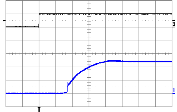
Fig. 1.2V.4: Turn-on transient at full rated load current (resistive) plus 20,000 \mu F at V_{in} = 48 V, triggered via ON/OFF pin. Top trace: ON/OFF signal (5 V/div.). Bottom trace: output voltage (0.5 V/div.). Time scale: 1 ms/div.
