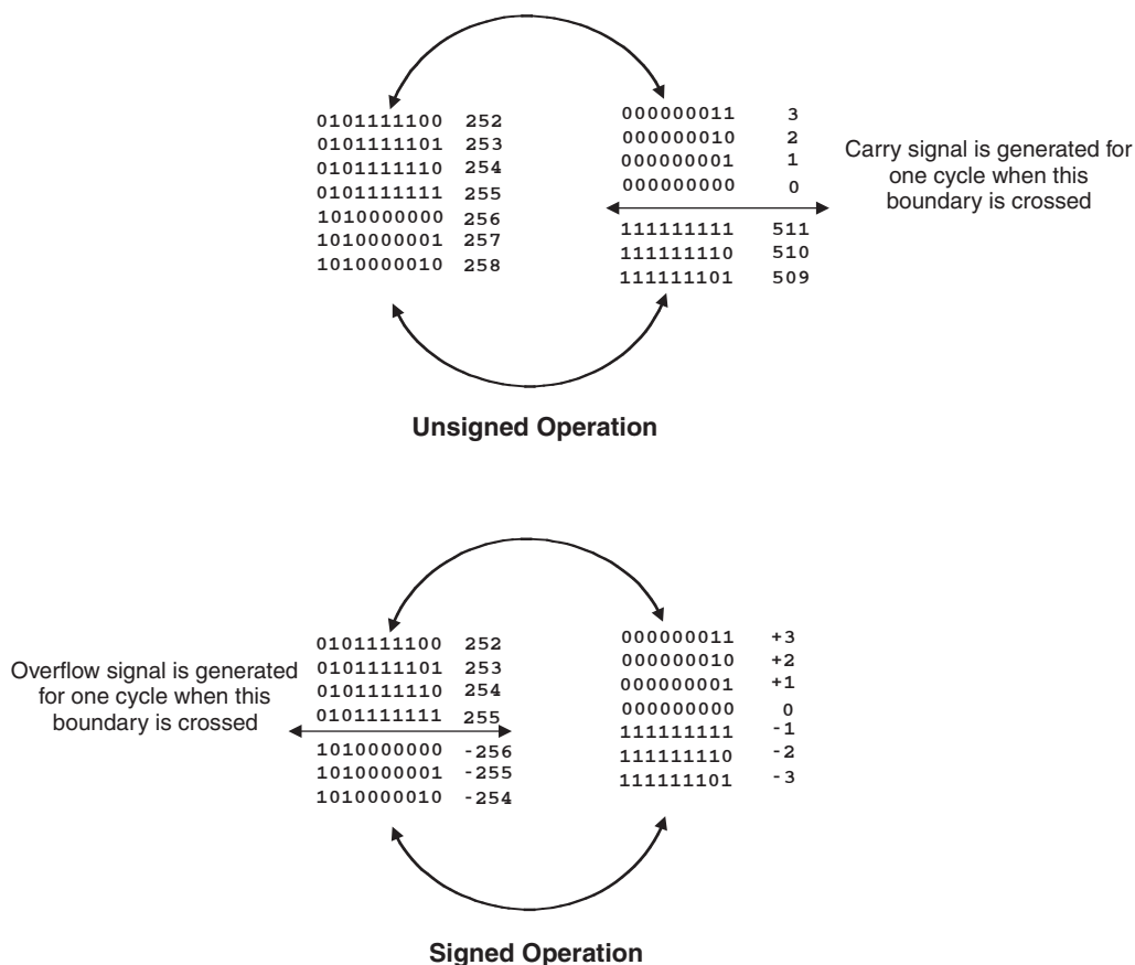
Figure 2-27. Accumulator Overflow/Underflow
