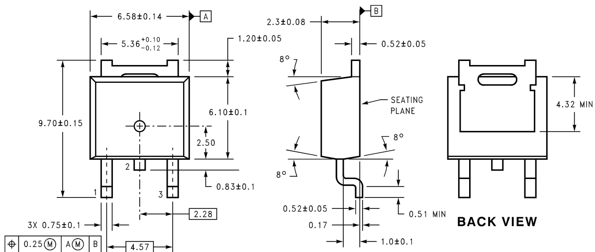
DIMENSIONS ARE IN MILLIMETERS D-Pak Package Order Number LP2950CDT-3.0, LP2950CDT-3.3, or LP2950CDT-5.0 NS Package Number TD03B
