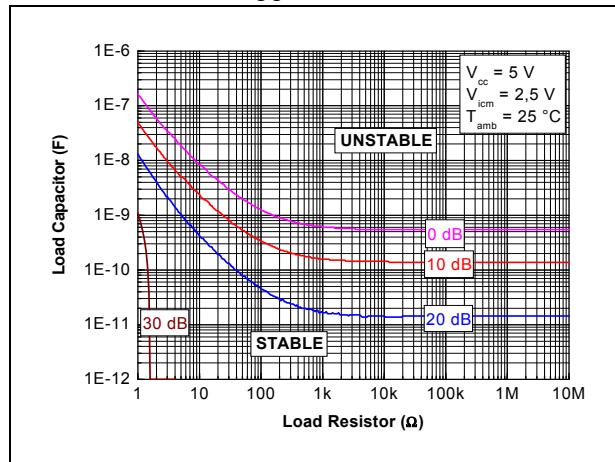
Figure 19. Gain margin according to the output load, at V_{CC}=5\text{ V} and T=25\text{ °C}
