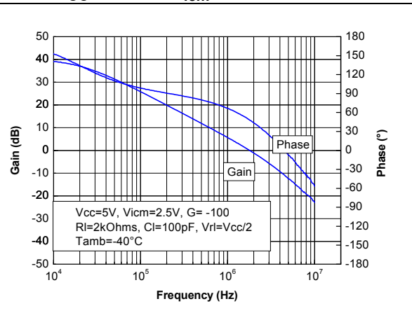
Figure 16. Voltage gain and phase vs. frequency at V_{CC}=5\text{ V} and V_{icm}=2.5\text{ V} at T=-40^\circ\text{C}
