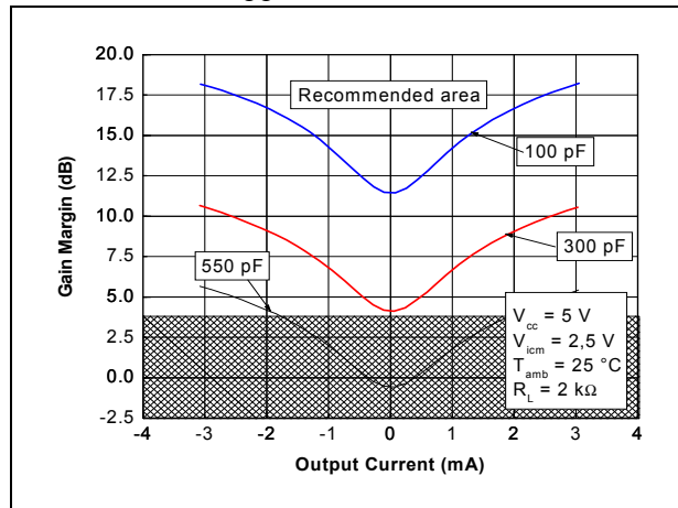
Figure 21. Gain margin vs. output current, at V_{CC}=5\text{ V} and T=25\text{ °C}
