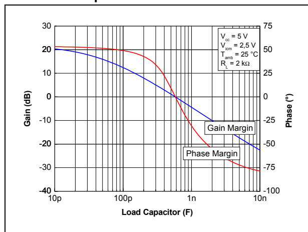
Figure 23. Phase and gain margins vs capacitive load at = 25\text{ °C}
