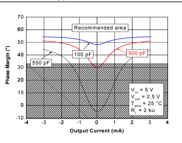
Figure 22. Phase margin vs. output current, at V_{CC}=5\text{ V} and T=25\text{ °C}
