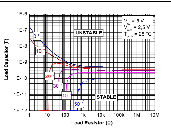
Figure 20. Phase margin according to the output load, at V_{CC}=5\text{ V} and T=25\text{ °C}
