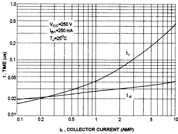
TURN-ON TIME
