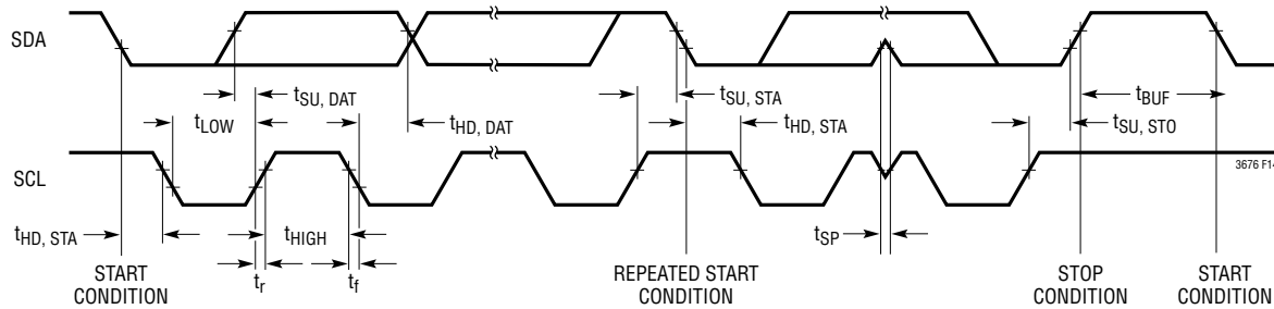
Figure 14. LTC3676 I 2 C Serial Port Timing
