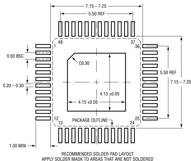
LXE Package 48-Lead Plastic Exposed Pad LQFP (7mm × 7mm) (Reference LTC DWG #05-08-1927 Rev 0) Exposed Pad Variation AA
