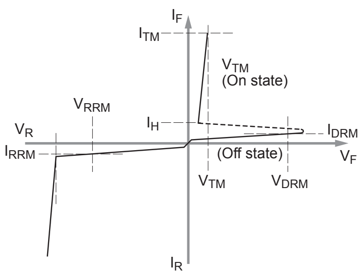
Voltage-Current Characteristic
