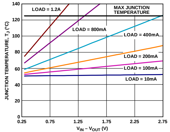
Figure 40. 500 mm 2 of PCB Copper, T_A = 50^\circ\text{C} , LFCSP
