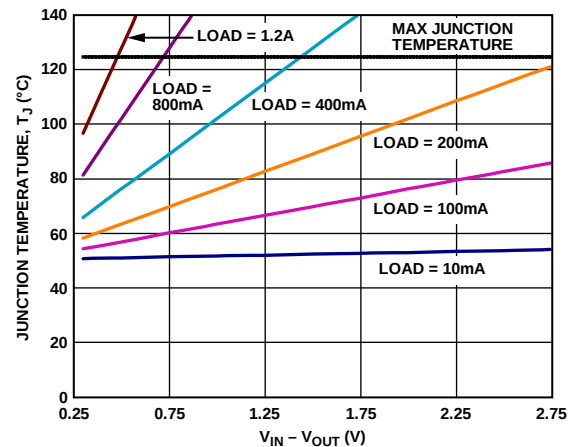
Figure 41. 0 mm 2 of PCB Copper, T_A = 50^\circ\text{C} , LFCSP
