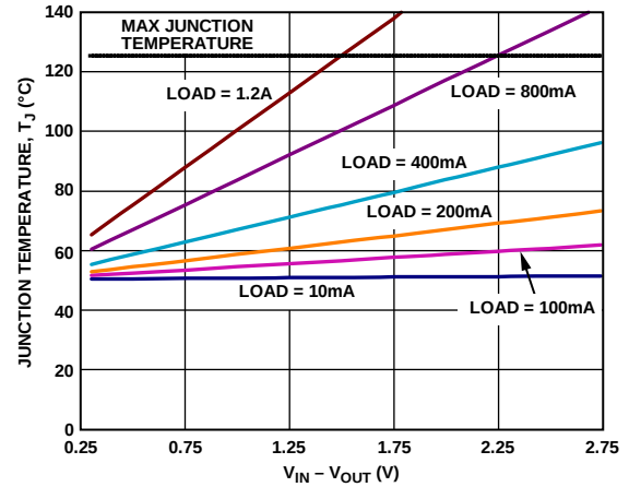
Figure 39. 6400 mm 2 of PCB Copper, T_A = 50^\circ\text{C} , LFCSP
