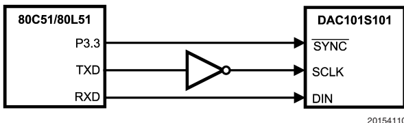
FIGURE 6. 80C51/80L51 Interface
