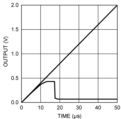
Power-On Reset
