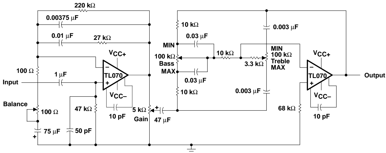
Figure 25. IC Preamplifier
