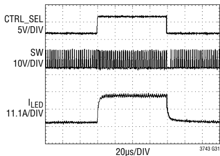
LED Current Waveforms (3000:1) 2A to 20A
