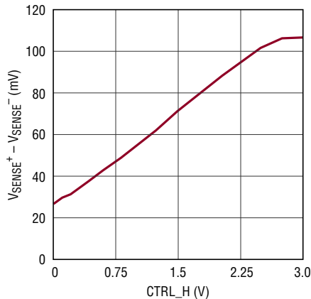
Overcurrent Threshold
