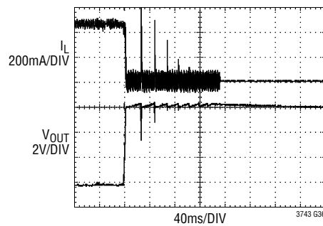
Overvoltage Lockout Operation With Open-Load Condition
