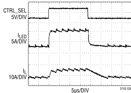
LED Current Waveforms (2000:1) 3A to 10A
