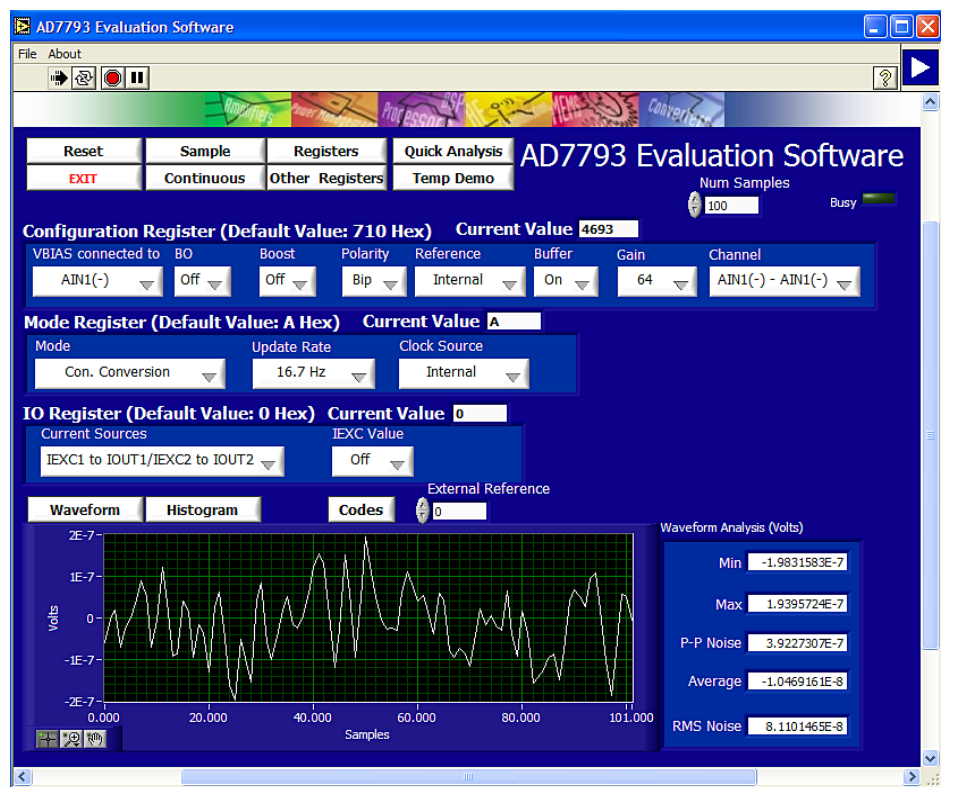
Figure 4. AD7793 Evaluation Software Registers Window
