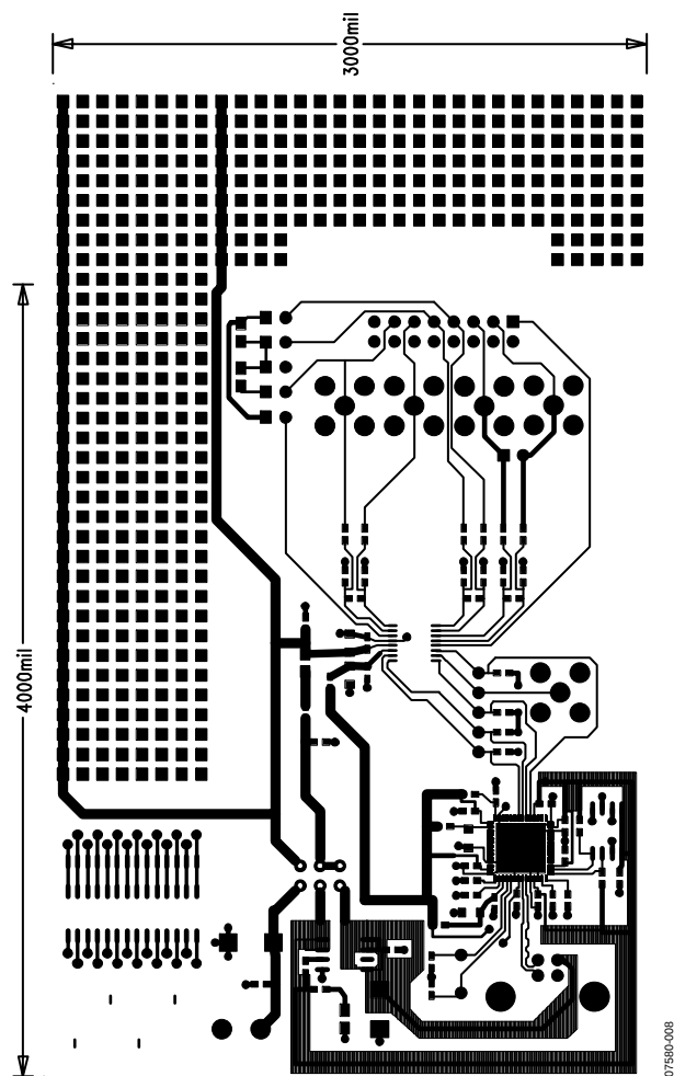
Figure 8. AD7793 Evaluation Board—Solder Side View
