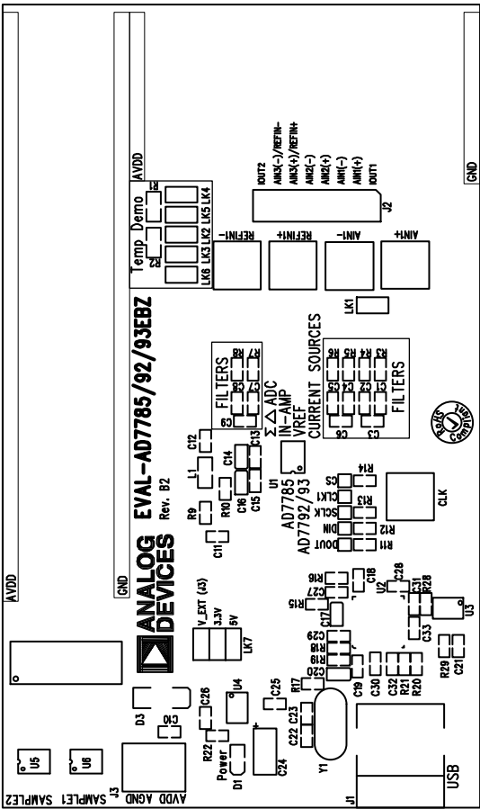
Figure 9. AD7793 Evaluation Board—Component Side View
