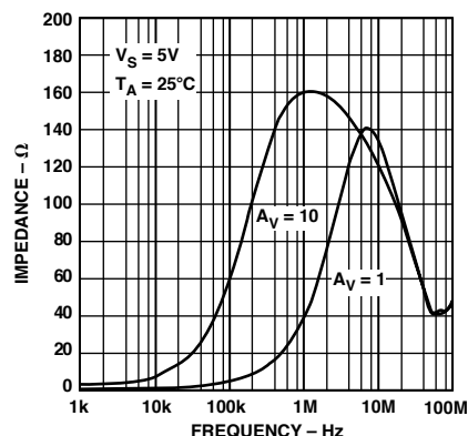
Figure 14. Closed-Loop Output Impedance vs. Frequency
