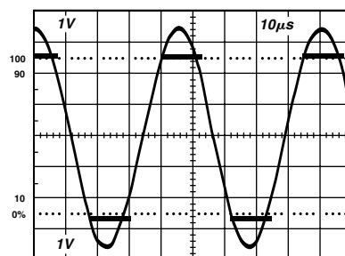
Figure 31. No Phase Reversal
