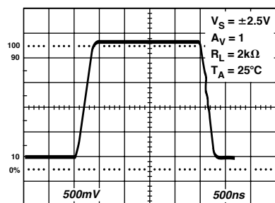
Figure 29. Large Signal Transient Response
