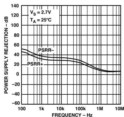
Figure 19. Power Supply Rejection vs. Frequency
