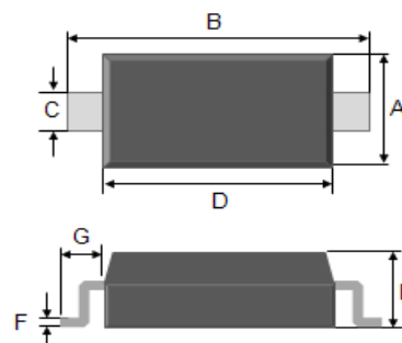
SOD-323
