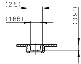
SECTION X-X
