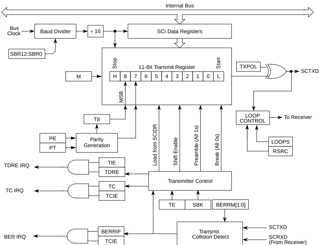
Figure 12-16. Transmitter Block Diagram
