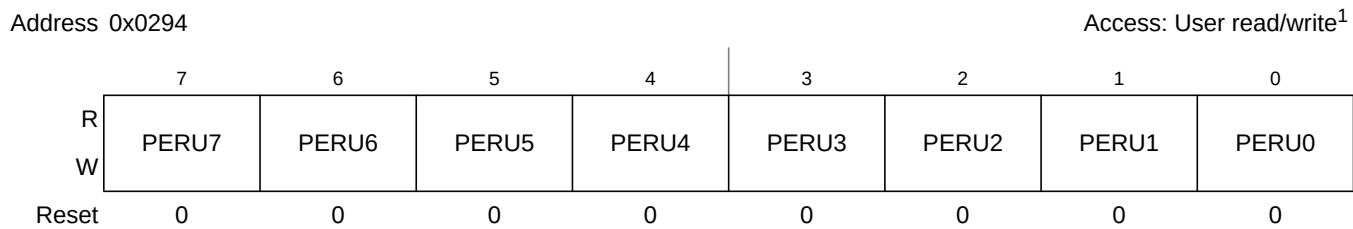
Figure 2-75. Port U Pull Device Enable Register (PERU)
