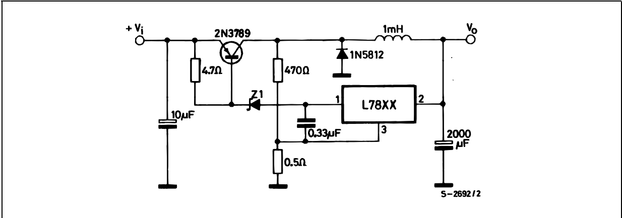
Figure 27: Switching Regulator
