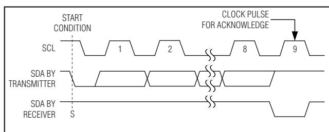
Figure 5. Acknowledge
