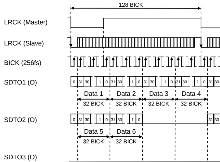
Figure 45. Mode 27/31 Timing (TDM128 Mode, I 2 S Compatible)
