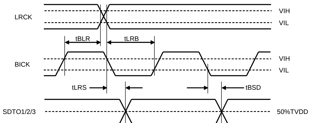
Figure 19. Audio Interface Timing (Normal Mode &amp; Slave Mode: 8 kHz ≤ fs ≤ 216 kHz)
