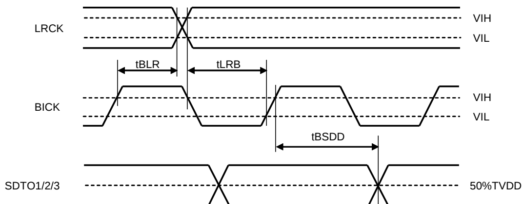
Figure 20. Audio Interface Timing (Normal &amp; Slave Mode: fs=384 kHz, 768 kHz)
