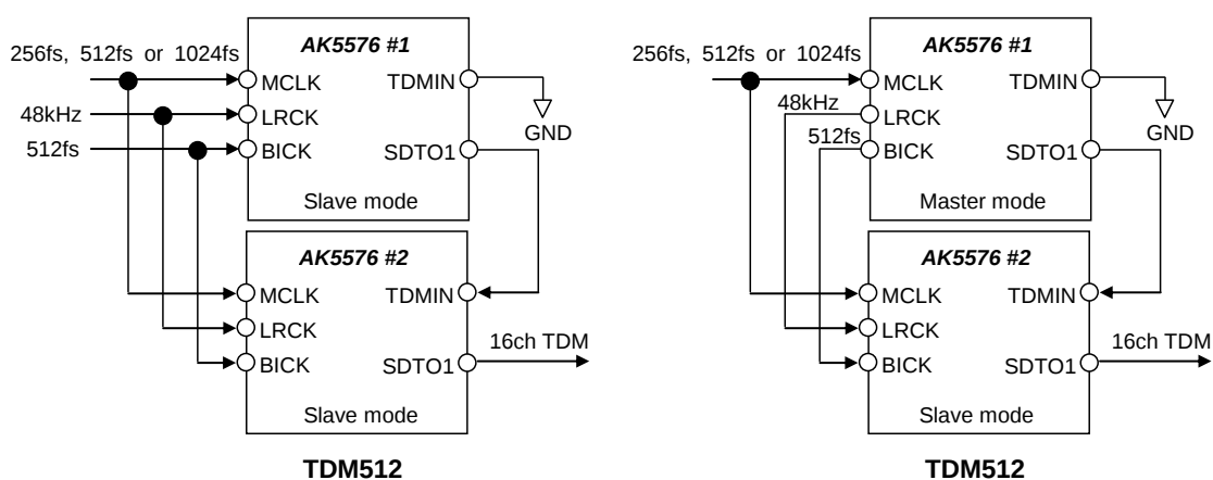
Figure 29. Cascade Connection
