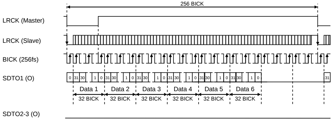
Figure 49. Mode 35/39 Timing (TDM256 Mode, I²S Compatible, 32-bit)
