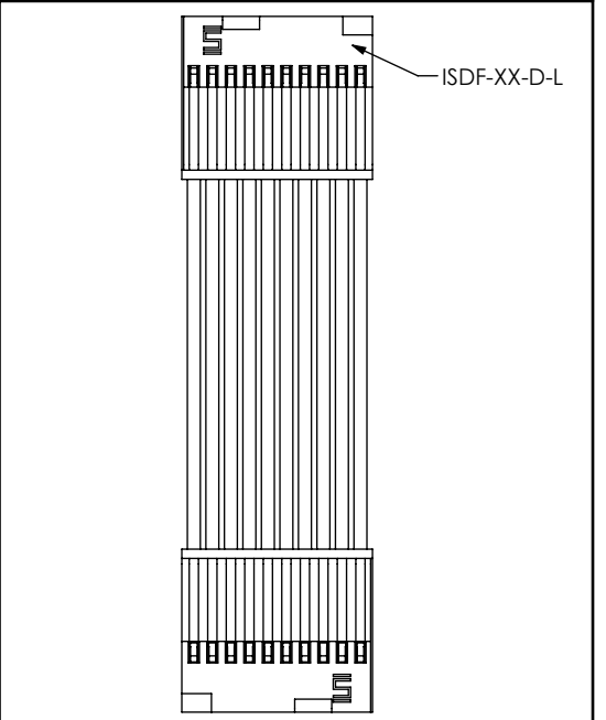
FIG 4 -DL: DOUBLE END FRICTION LOCK SFSDX-10-28-XX-XX.XX-DL-NUS SHOWN (SAME AS FIG 1, UNLESS OTHERWISE STATED)
