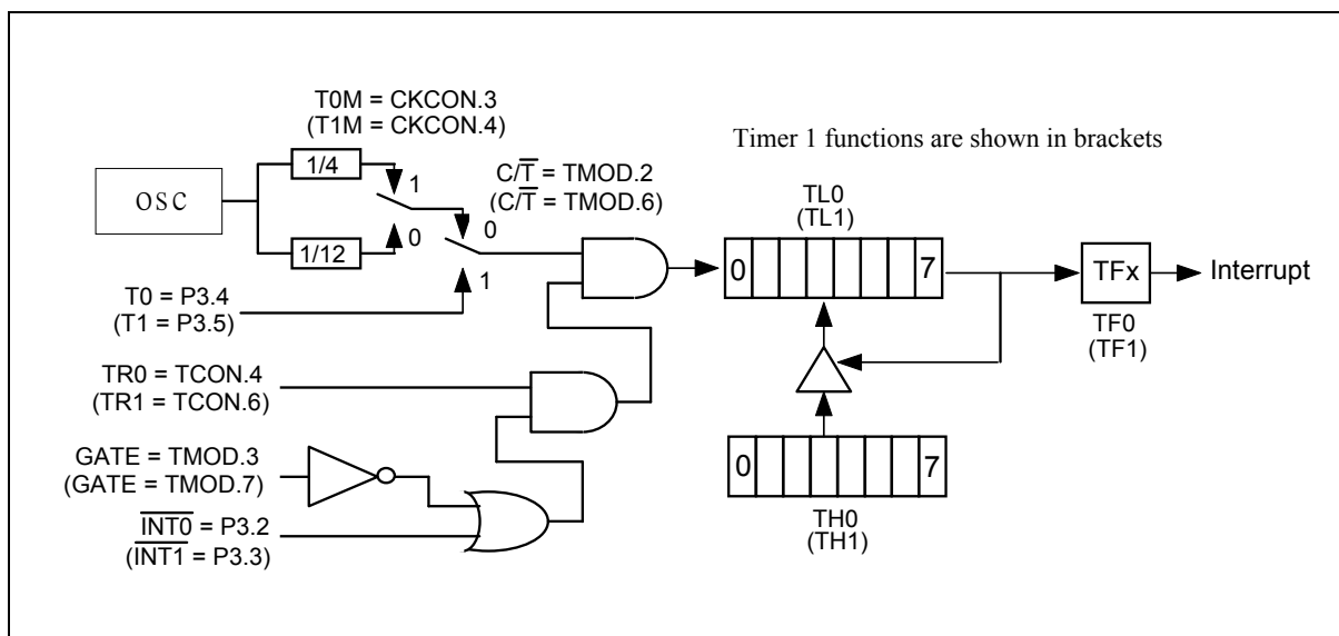
Figure 10-2 Timer/Counter Mode 2
