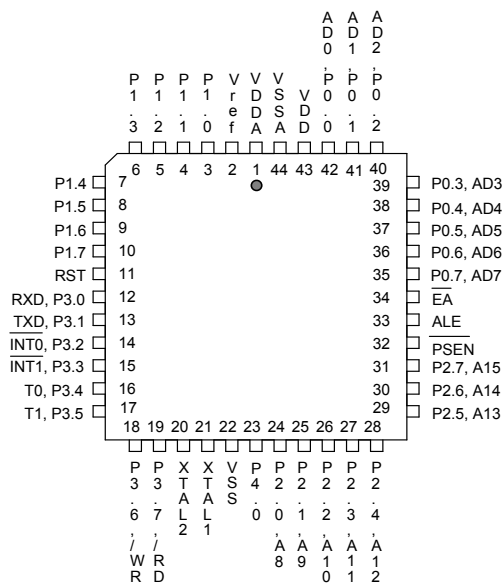
44-Pin PLCC
