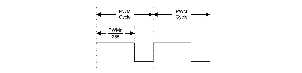
Figure 13-2 PWM Duty Cycle
