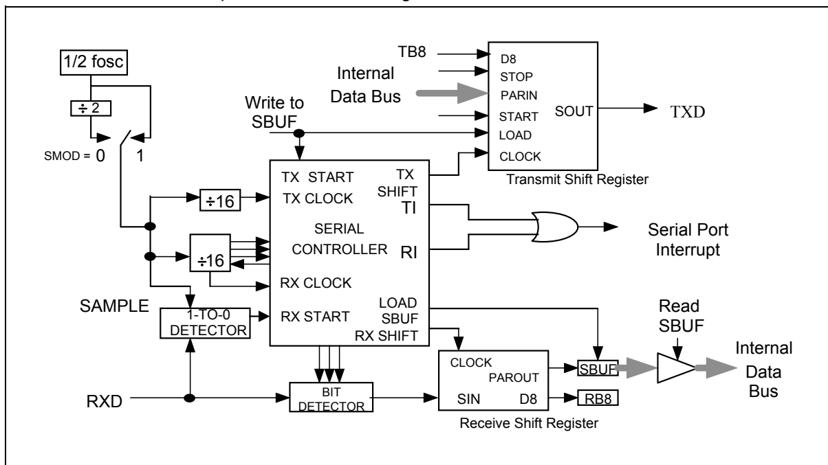
Figure 12-3 Serial Port Mode 2
