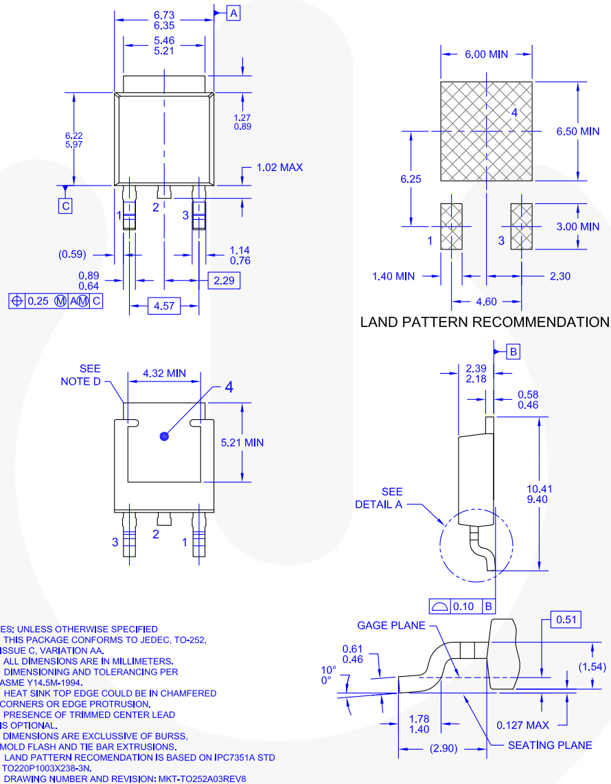
Figure 9. TO252 (D-PAK), MOLDED, 3-LEAD, OPTION AA&amp;B (ACTIVE)
