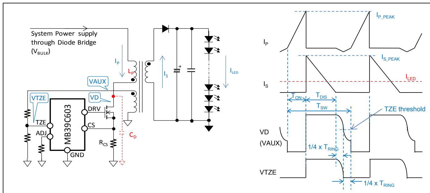
Figure 8-1 LED Current Control Waveform
