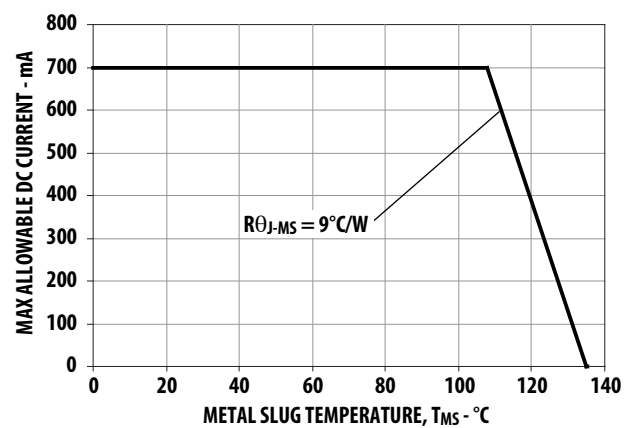
Figure 12. Maximum Forward Current vs. Metal Slug Temperature. Derated based on T_{JMAX} = 135^\circ\text{C} , R_{\theta MS} = 9^\circ\text{C/W}
