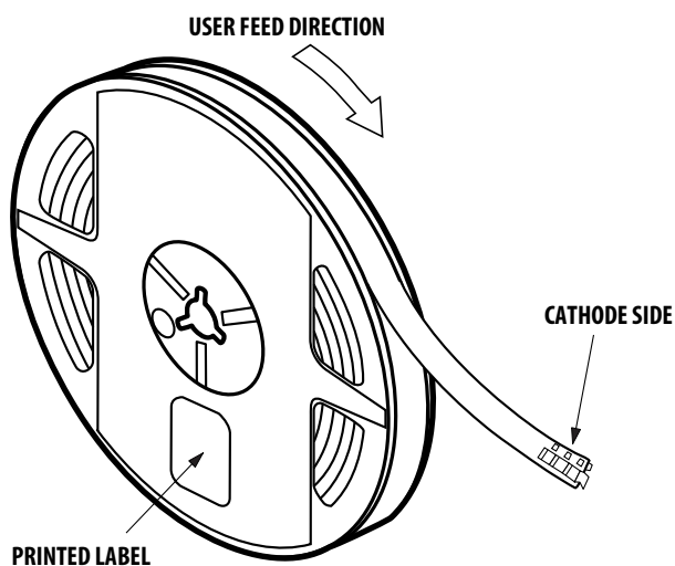
Figure 21. Reeling Orientation
