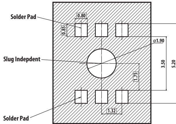
Figure 13. Recommended soldering land pattern
