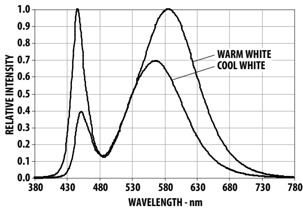
Figure 2. Relative Intensity vs. Wavelength for Cool White and Warm White
