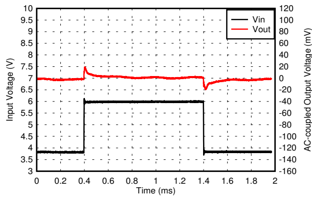
Figure 5-25. 3.3-V Line Transient
