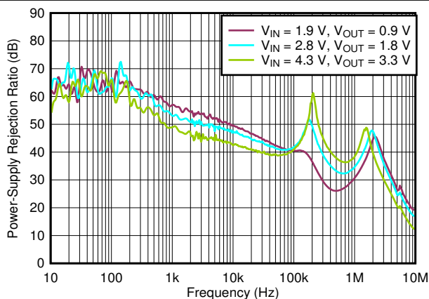
Figure 5-33. PSRR vs Frequency and V_{IN}
