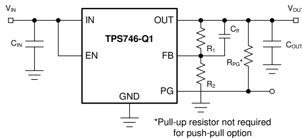
Figure 7-1. Adjustable Operation
