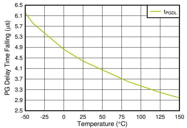
Figure 5-20. t_{PGDL} vs Temperature
