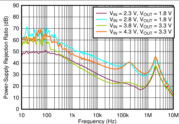
Figure 5-34. PSRR vs Frequency and V_{IN}
