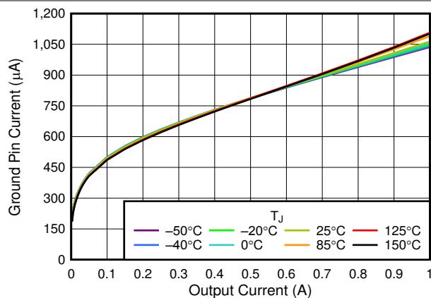
Figure 5-8. I_{GND} vs I_{OUT}
