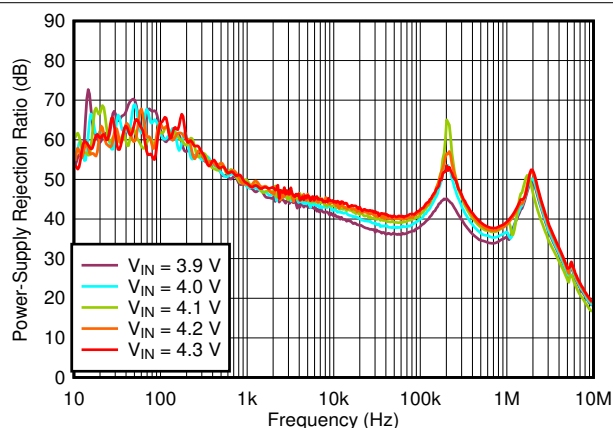
Figure 5-32. PSRR vs Frequency and V_{IN}
