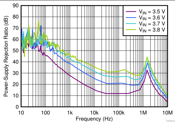
Figure 5-31. PSRR vs Frequency and V_{IN}
