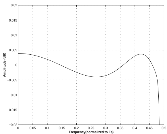
Figure 16. Single-Speed (fast) Passband Ripple
