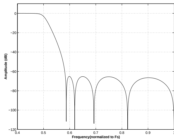
Figure 17. Single-Speed (slow) Stopband Rejection
