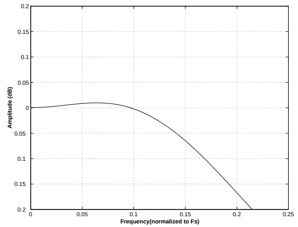
Figure 32. Quad-Speed (fast) Passband Ripple
