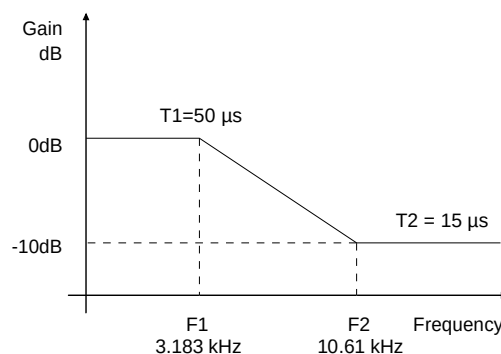
Figure 11. De-Emphasis Curve
