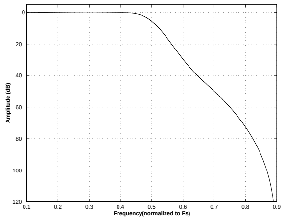
Figure 34. Quad-Speed (slow) Transition Band
