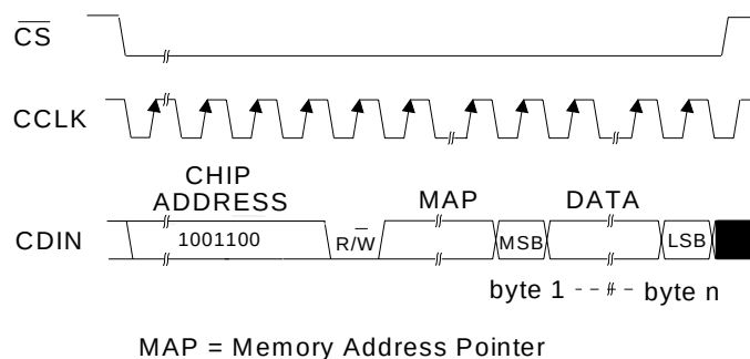
Figure 10. Control Port Timing, SPI mode
