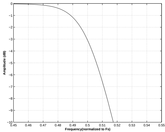
Figure 19. Single-Speed (slow) Transition Band (detail)
