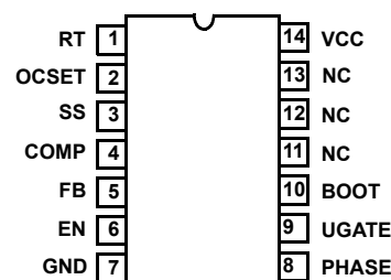
HIP6013 (SOIC) TOP VIEW
