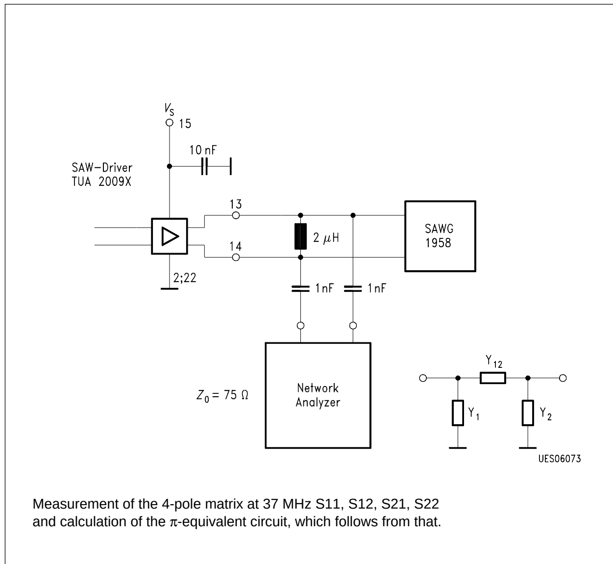
Test Circuit 4
