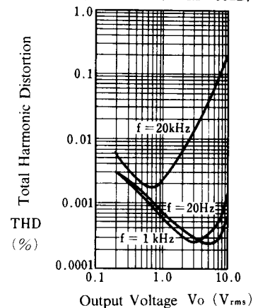
Total Harmonic Distortion vs. Output Voltage
