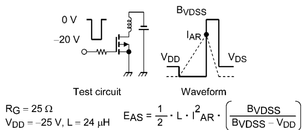
Fig. 8.15 Test Circuit/Waveform
